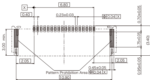
Recommended PCB Dimensions
