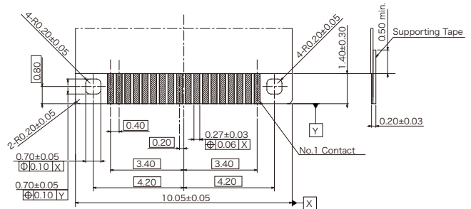
Recommended FPC Dimensions
